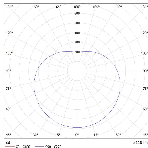
Lucis ZK.P1.500.X POLARIS ZK LED / LDC (Polar)
